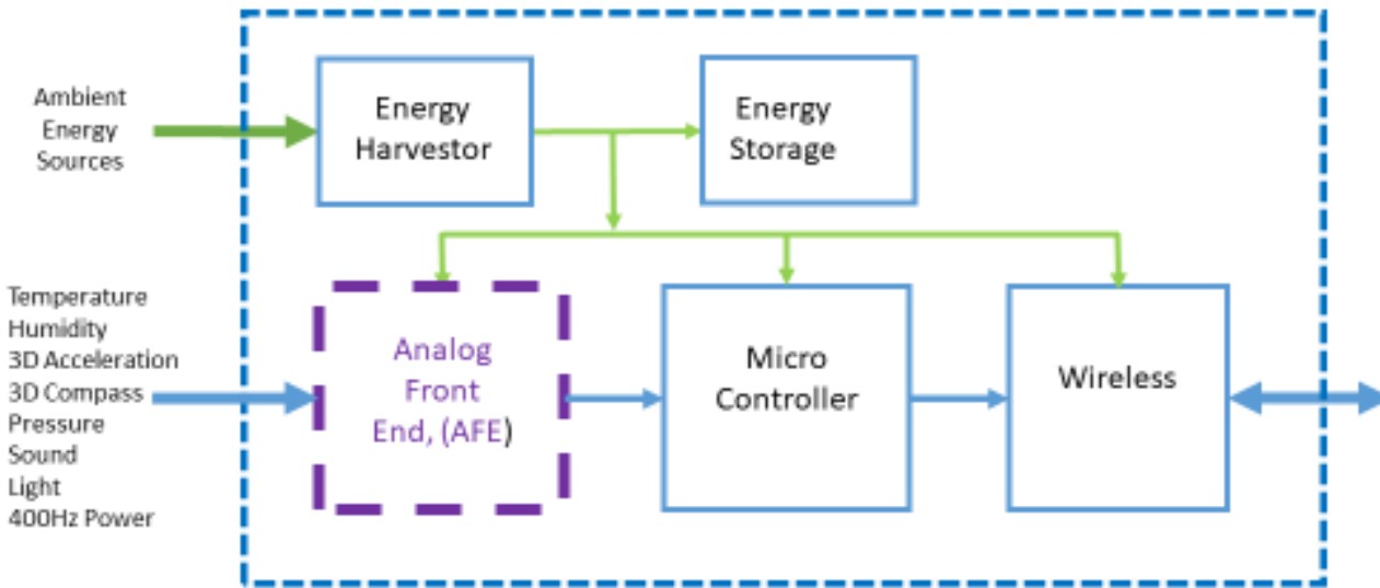
Energy-harvesting-powered system
